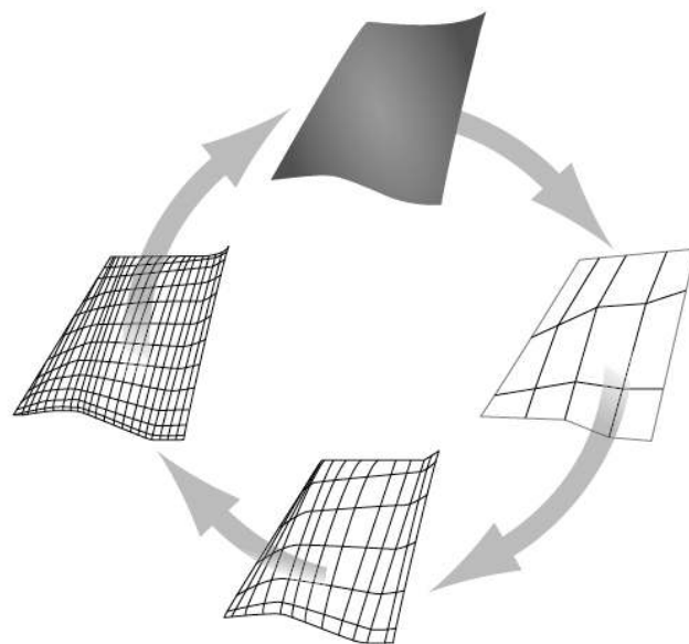
Figure 13 Quantum gauge fields are first described on a lattice, after which one takes the limit of small lattice spacing to analyse the quantum theory in the continuum.
