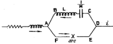
Figure 1 Circuit diagram of the singing arc, Poincaré [31, p. 390]
