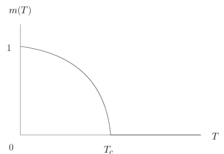
Figure 1 Spontaneous magnetisation: the magnetisation m(T) as a function of the temperature T for a typical configuration of the spins; m(T) is the difference between the number of up-spins and the number of down-spins divided by the total number of spins. The characteristic feature of ferromagnets is that there is a critical temperature , T_c , below which the spins exhibit collective behaviour in that a majority of them point in the same direction (either a majority up or a majority down). By symmetry, configurations with the opposite magnetisation -m(T) are equally likely.
