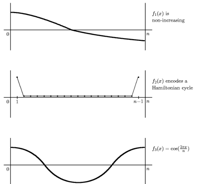
Figure 7 The generating functions for the three symmetric Toeplitz matrices
