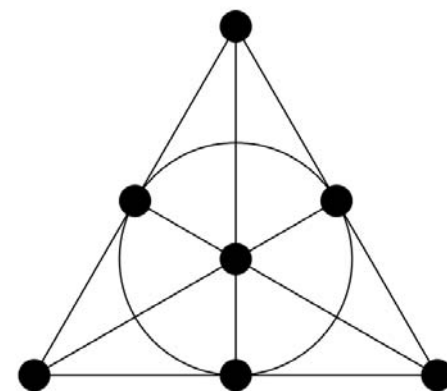
Figure 1 Fano plane.
