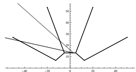
Figure 2 The number of reflections of a ray is the same as the number of reflected cups it passes. So in this example the red ray (dark grey) is reflected once and the blue ray (light grey) twice.
