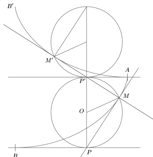
Figure 4 The construction of Huygens amplitude invariant pendulum. The curve AB is (half) a cycloid, along which the pendulum mass M , attached to the string B'M , is supposed to move.
